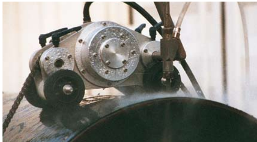
Demolition of rubber coated pipe elements using the Eco Top Cutter
